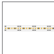
LED-Leiste HQ-210E3 24V 9.6 W/m Ref: HQ-210E3
